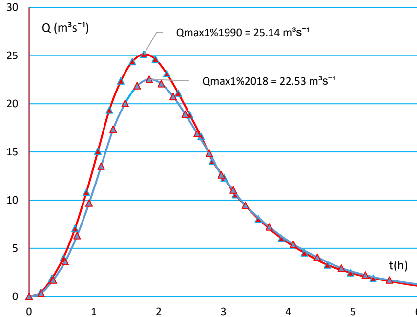
Figure 5. Peaks of torrential floods with 100 return period of the Ravna reka in 1990 and 2018
