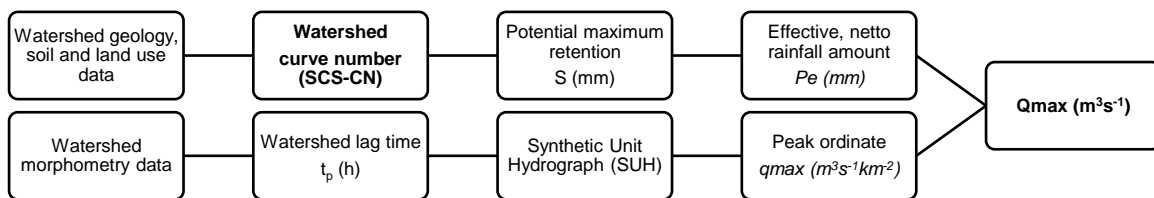
Figure 2. Description of the SCS-UH methodology for reconstruction of the maximal discharges (Source: Petrović et al. 2021)
